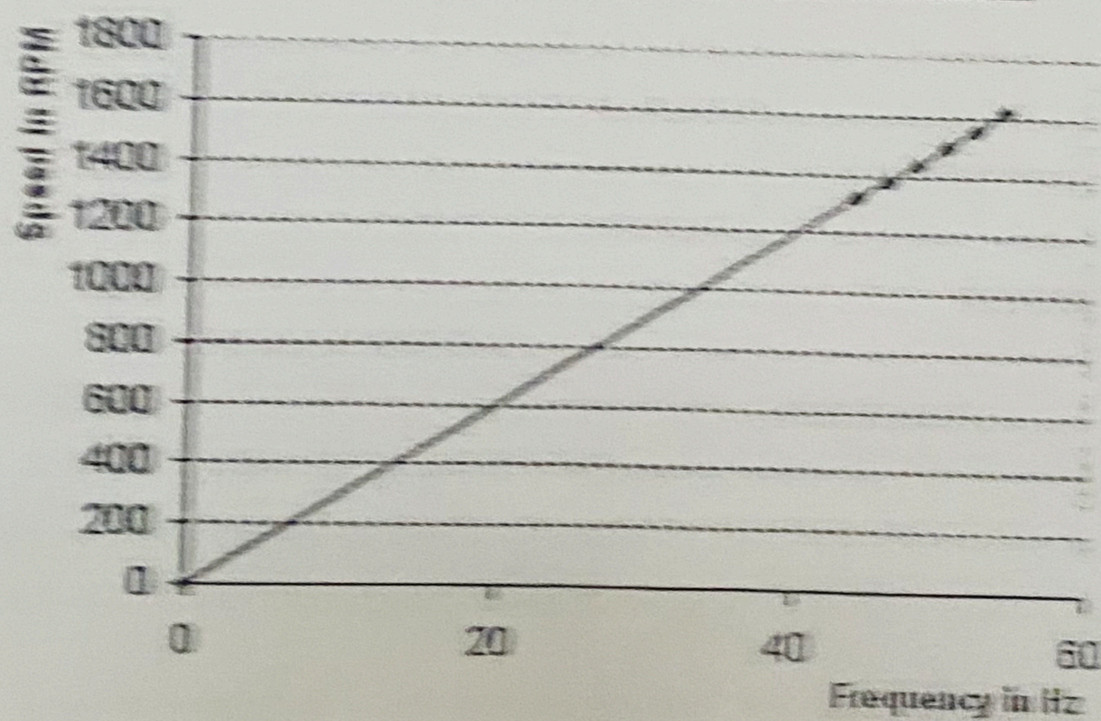
Speed Vs frequency curve on load
